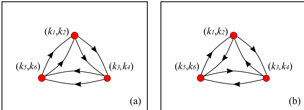
Figure 6. (Color online) Oriented connected graphs used for the evaluation of the third cumulant. (a): same internal and external orientations of the edges (nonvanishing “current”). (b): opposite internal and external orientations of the edges (vanishing “current”).
