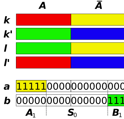
Figure A1. (Color online) Graphic representation of the combination of binary strings contributing to sum (A.2).
