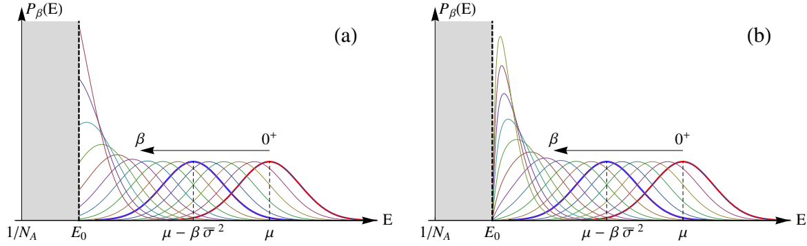
Figure 2. (Color online) Qualitative sketch of Eq. (34), at fixed N_A , in arbitrary units. The energy density function is distributed around \mu with standard deviation \bar{\sigma} at \beta = 0 (first bell-shaped curve at the right in both panels) and moves toward E_0 when \beta increases. In each panel, from right to left, \beta changes in constant steps. The probability density rigidly shifts with \beta , for \beta \lesssim N^{7/2 - \log_2 3} ; see Eq. (133) and following discussion. Note that both E_0, \mu are O(N^{-1/2}) . In (a) P_0(E_0) \neq 0 ; in (b) P_0(E_0) = 0 .
