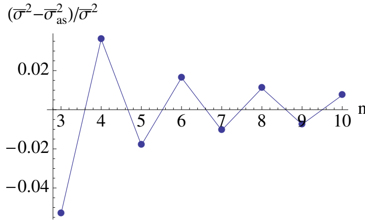
Figure 4. (Color online) Difference between the analytic value of second cumulant, computed according to Eq. (104) with f_2 given by (99), and its asymptotic limit, obtained by substituting (105) into Eq. (104). The approximation is valid within a few percent even for n = 3 .
