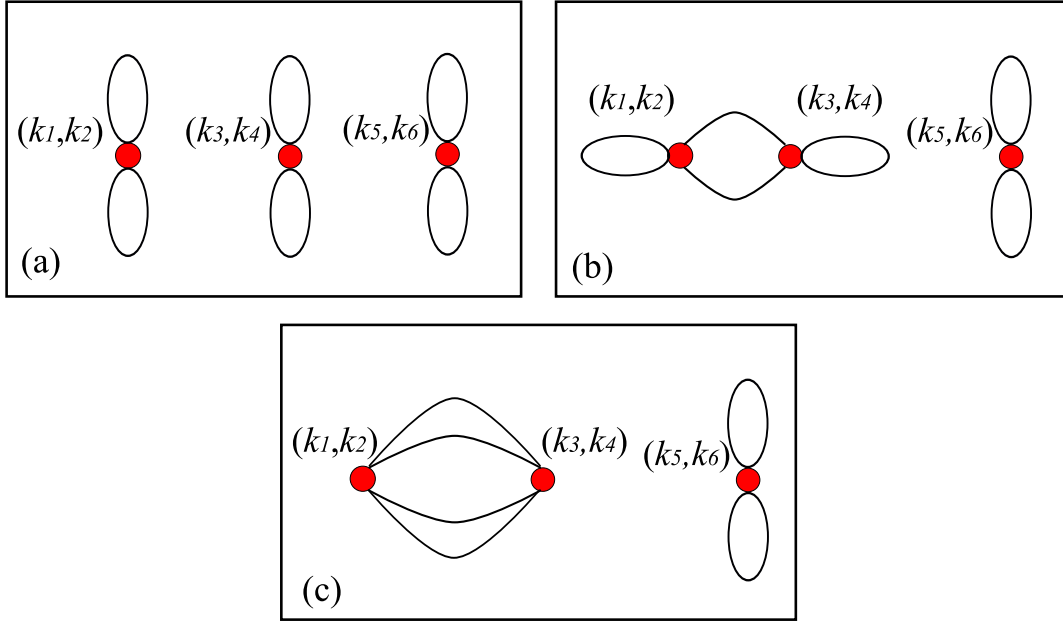
Figure 7. (Color online) Disconnected graphs used for the evaluation of the third cumulant. (a): six loops. (b): four loops. (c): two loops.
