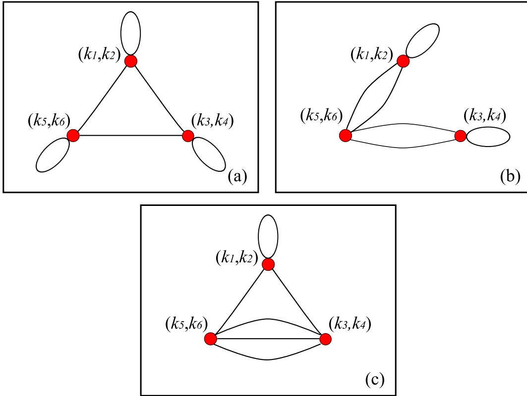
Figure 5. (Color online) Non-oriented connected graphs used for the evaluation of the third cumulant. (a): three ears. (b): two ears. (c): one ear.
