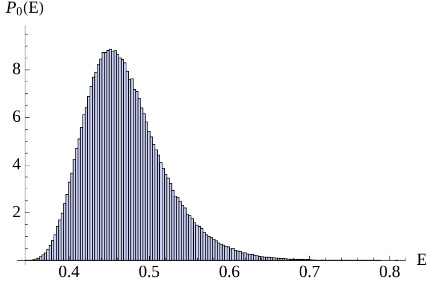
Figure 1. (Color online) Probability density function P_0(E) for n = 4 . The distribution has been obtained from 5 \times 10^5 typical states. The binning is 3 \times 10^{-3} and the integral is equal to 1.
