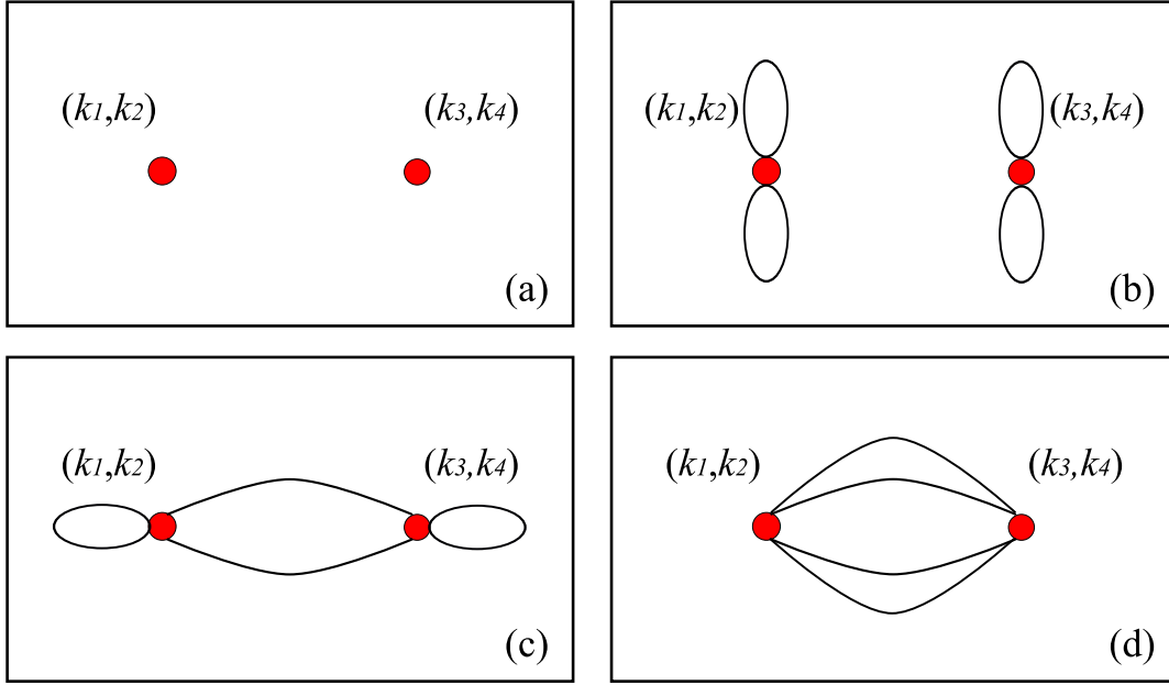
Figure 3. (Color online) Graphs used for the evaluation of the second cumulant (75). (a): empty diagram. (b): graph with no links between the left and right pairs. (c): graph with two links between the left and right pairs. (d): graphs with four links between the left and right pairs.
