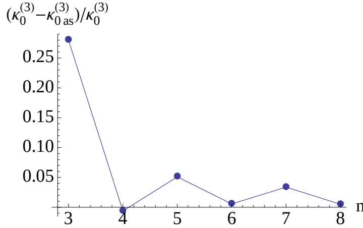
Figure 8. (Color online) Difference between the analytic value of third cumulant, computed according to Eq. (125) with f_2 , f_3^{(0)} and f_3^{(1)} given by (99), (120), (120), and their asymptotic limits, obtained by substituting (105), (126), (127) into Eq. (125). The approximation is valid within a few percent for n \geq 4 .
