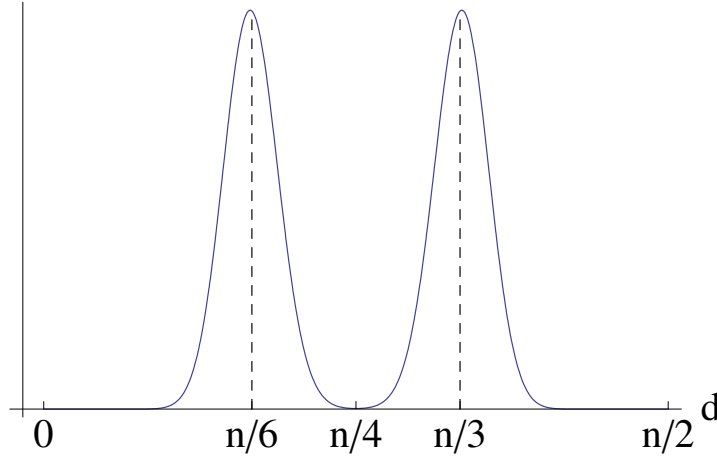
Figure B1. (Color online) d -dependence of the terms \binom{n_A}{d} \binom{n_{\bar{A}}}{d} 2^{n/2} [4^{n/4-d} + 4^{-(n/4-d)}] in the sum (B.11).
