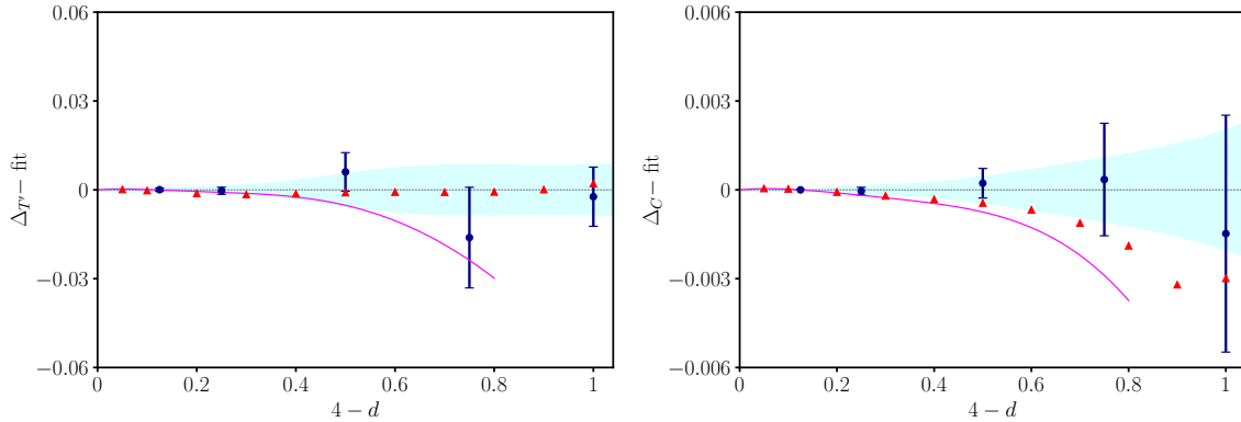
Figure 16: Comparison of scaling dimensions minus best fit for T' , C fields: bootstrap (blue round points), navigator method [20] (triangle red points) and unresummed epsilon-expansion [26, 31, 57, 58] (magenta solid line).
