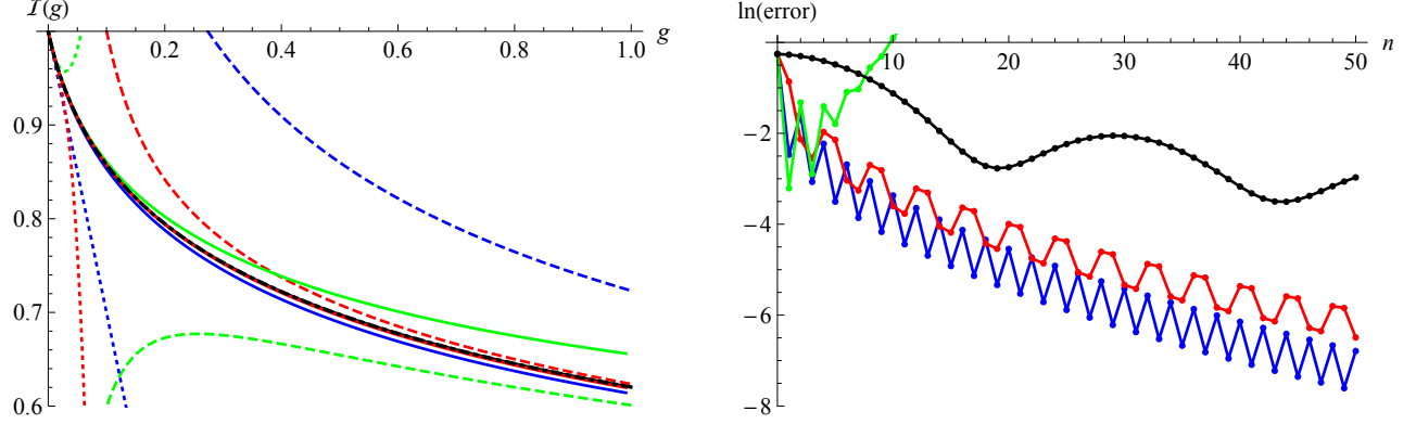
Figure 21: Left: The function \mathcal{I}(g) (black, thick, dot-dashed) and its diverse approximations: Dotted for the series expansion at order 1 (blue), 2 (green), and 3 (red). Solid for the resummed series at the same order. Dashed for the large- g expansion (same color code). Right: Deviation of the resummed series (B.9) from the exact result (B.5) for g = 10 as a function of n , assuming one knows t_{bc} only approximately. In blue for t_{bc} = -1/16 (the exact result), in red t_{bc} = -1/32 (a conservative guess), in black t_{bc} = -1/1000 (much too small). Resummation with t_{bc} = -1/15 (green) does not work. We see that conform to expectations, taking a too small value for -t_{bc} , the series converges more slowly, while taking a too large value of -t_{bc} the series does not converge.
