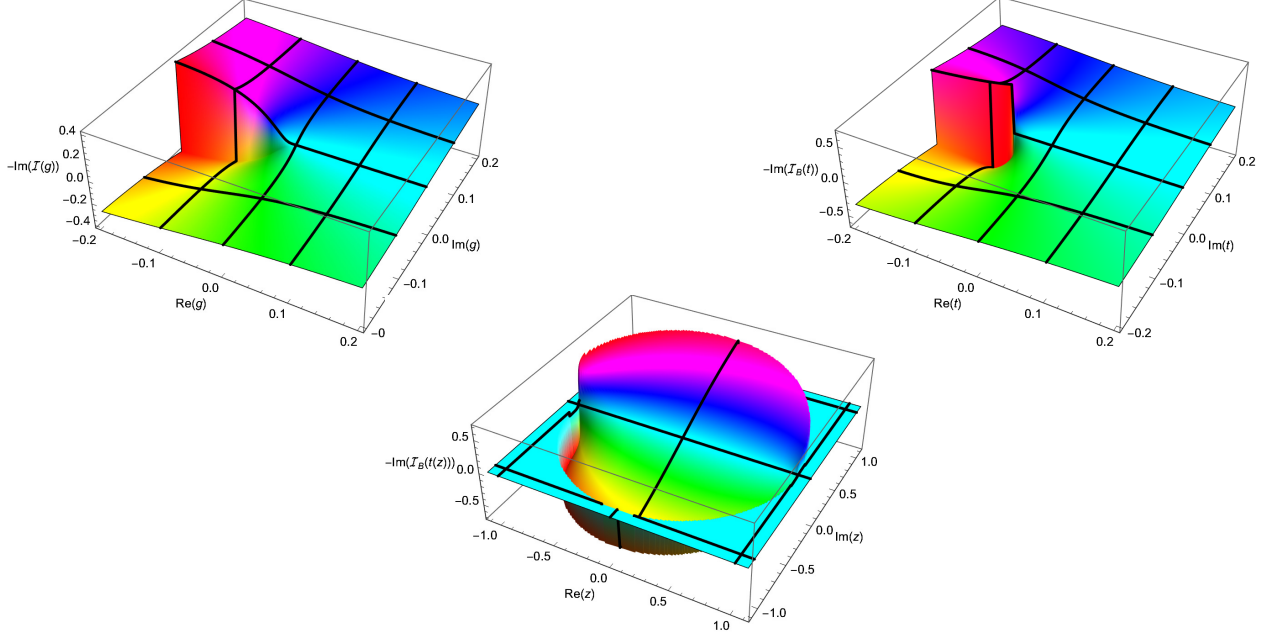
Figure 20: The branch cut in \mathcal{I}(g) (top left) and \mathcal{I}_B(t) (top right). While the former starts at g = 0 , the latter is moved to g = -1/16 . The lower plot shows \mathcal{I}_B(t(z)) , which now has a branch-cut singularity at |z| = 1 . (We set \mathcal{I}_B(t(z)) to 0 outside the disc |z| \geq 1 .)
