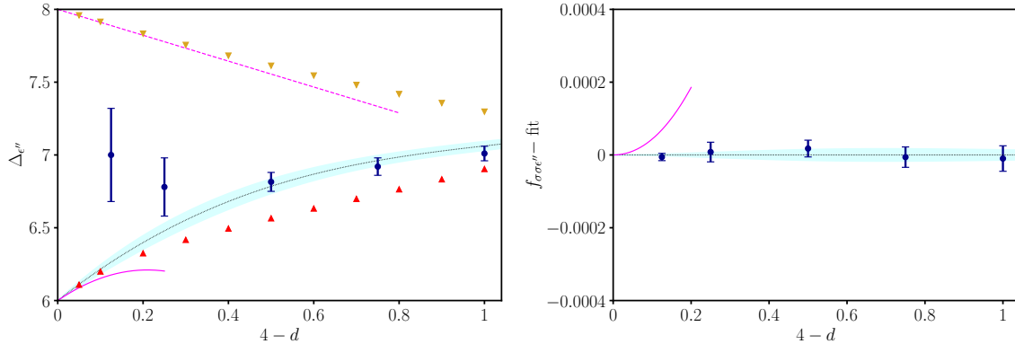
Figure 19: Scaling dimension and structure constant of the would-be \epsilon'' operator in our bootstrap spectrum (blue circles). Upward red and downward gold triangles represent navigator results for \epsilon'' and \epsilon''' [20]. The solid and dashed magenta lines are the corresponding leading-order epsilon-expansion, which agree with the navigator results, but not ours.
