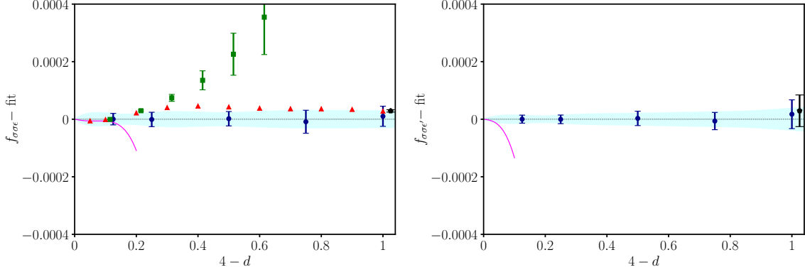
Figure 15: Comparison of f_{\sigma\sigma\epsilon} and f_{\sigma\sigma\epsilon'} minus best fit: bootstrap (blue circles), unresummed epsilon-expansion [29, 30, 57, 58] (magenta solid curve), 3-correlator bootstrap at d = 3 [46] (black pentagon). On the left we also report the resummed epsilon-expansion (green squares) and bootstrap navigator results [20] (red triangles).
