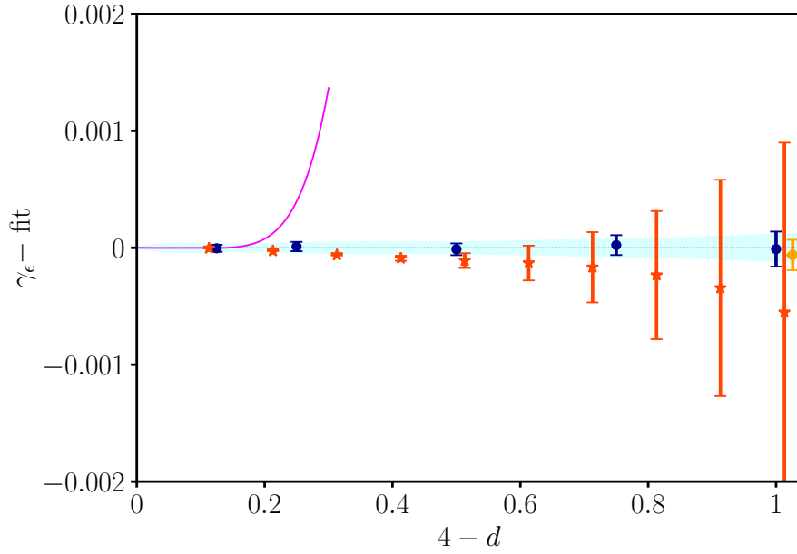
Figure 10: Comparison of \gamma_\epsilon minus best fit: bootstrap (blue circles), Self-Consistent resummed epsilon-expansion [39] (red stars), unresummed epsilon-expansion (magenta solid curve), d=3 Monte Carlo [42] (yellow rhombus).
