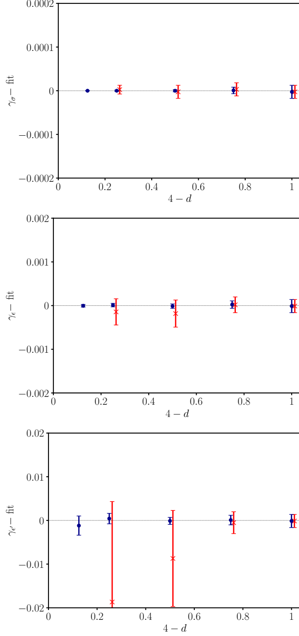
Figure 3: Old [19] (red crosses) and new (blue circles) bootstrap data for \gamma_\sigma, \gamma_\epsilon, \gamma_{\epsilon'} , minus the corresponding best fits. (The plots use the same scales as in Ref. [19]).
