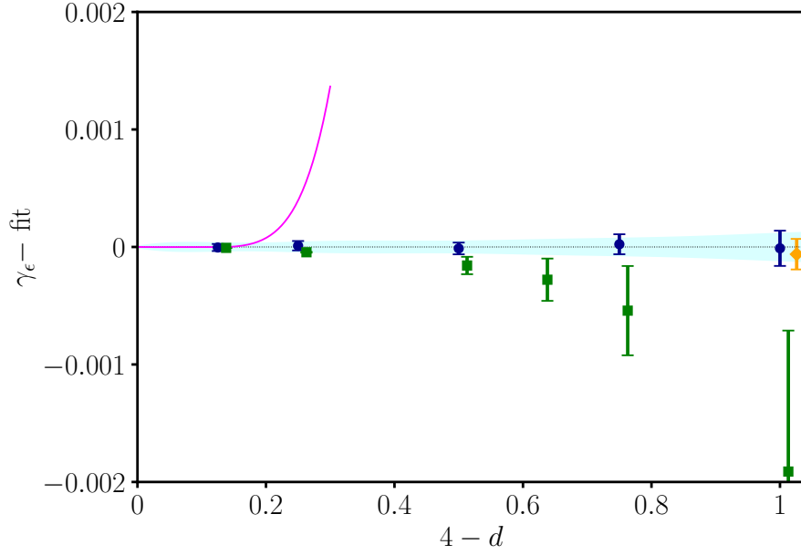
Figure 9: Comparison of \gamma_\epsilon data minus best fit: bootstrap (blue circles), Borel-resummed epsilon-expansion [38] (green squares), unresummed epsilon-expansion (magenta solid curve), d=3 Monte Carlo [42] (yellow rhombus). The cyan shaded area is the fit error as in earlier plots.
