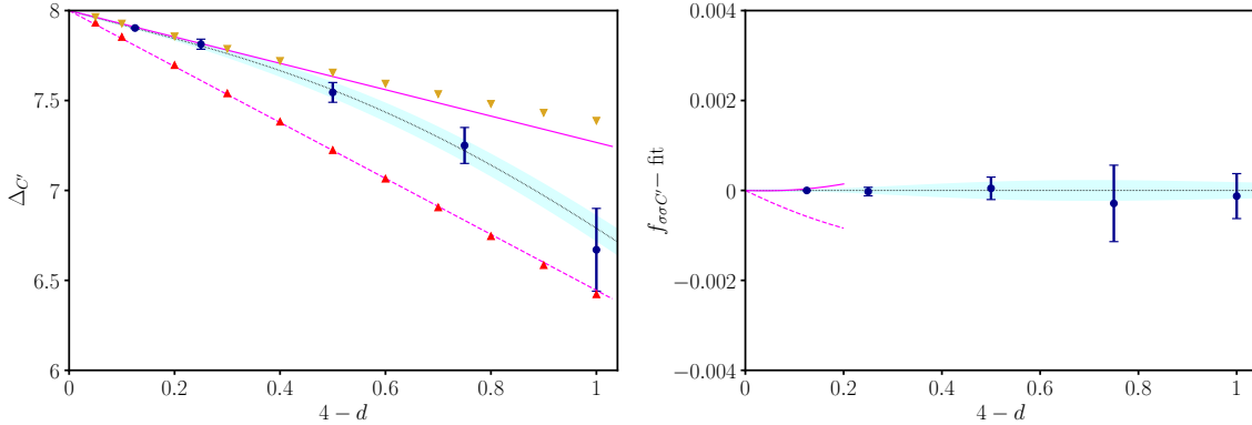
Figure 18: Scaling dimension and structure constant of would-be C' operator in our bootstrap spectrum (blue circles). Upward red and downward gold triangles represent navigator results for C' and C'_2 [20]. The dashed and solid magenta lines are the corresponding leading-order epsilon-expansion.
