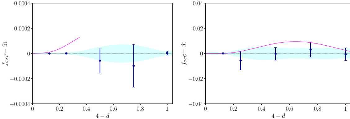
Figure 17: Behavior of structure constants f_{\sigma\sigma T'} and f_{\sigma\sigma C} (round blue points) compared with epsilon-expansion (magenta solid line) [57, 58].
