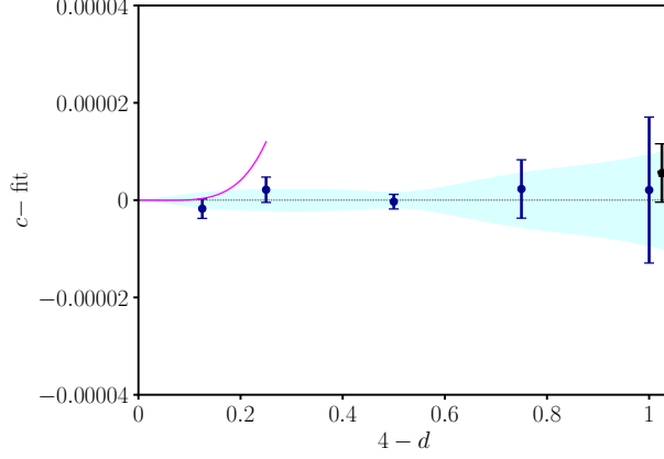
Figure 14: Comparison of c data minus best fit: bootstrap (blue circles), unresummed epsilon-expansion [57, 58] (magenta solid curve), 3-correlator bootstrap at d = 3 [46] (black pentagon).
