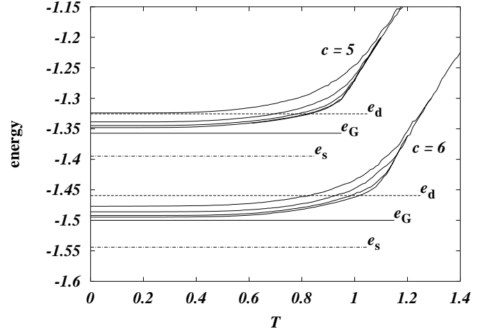
Fig. 6. 3-spin Ising model with fixed connectivity c , energy relaxation during slow simulated annealings. The 4 different full curves correspond to 4 cooling rates proportional to 1, 10^{-1}, 10^{-2}, 10^{-3} . The values for e_d , e_G and e_s are those reported in Table 1.
