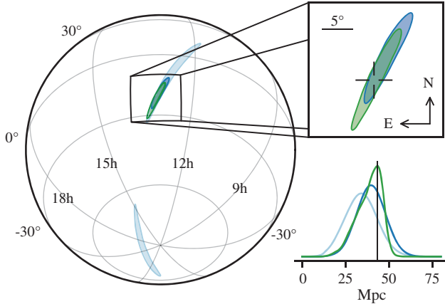
FIG. 3. Sky location reconstructed for GW170817 by a rapid localization algorithm from a Hanford-Livingston (190 deg 2 , light blue contours) and Hanford-Livingston-Virgo (31 deg 2 , dark blue contours) analysis. A higher latency Hanford-Livingston-Virgo analysis improved the localization (28 deg 2 , green contours). In the top-right inset panel, the reticle marks the position of the apparent host galaxy NGC 4993. The bottom-right panel shows the a posteriori luminosity distance distribution from the three gravitational-wave localization analyses. The distance of NGC 4993, assuming the redshift from the NASA/IPAC Extragalactic Database [89] and standard cosmological parameters [90], is shown with a vertical line.
