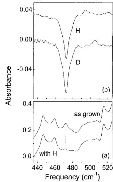
FIG. 3. Vibrational spectra showing the N mode for \text{GaAs}_{0.992}\text{N}_{0.008} samples measured at 4.2 K with a resolution of 2 \text{ cm}^{-1} . Spectra for an as-grown sample and a sample hydrogenated with a dose of 2 \times 10^{18} \text{ H}^+/\text{cm}^2 are shown in (a). Difference spectra for hydrogenated and deuterated (with dose 2 \times 10^{18} \text{ D}^+/\text{cm}^2 ) samples are compared in (b).
