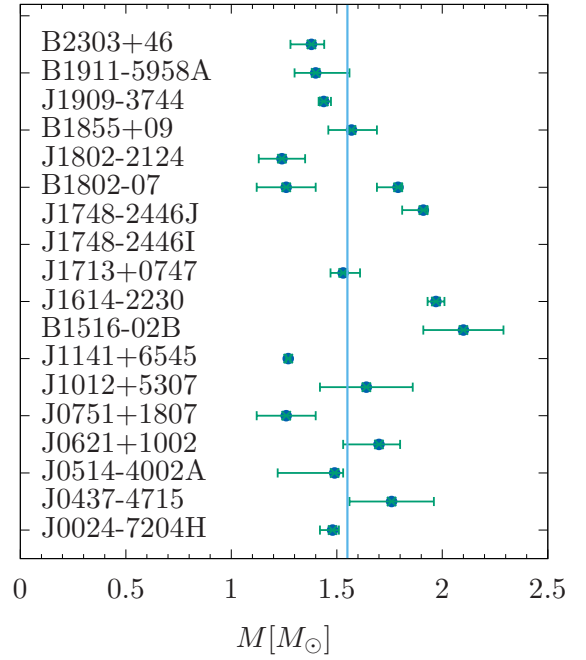
Neutron star-white dwarf binaries
