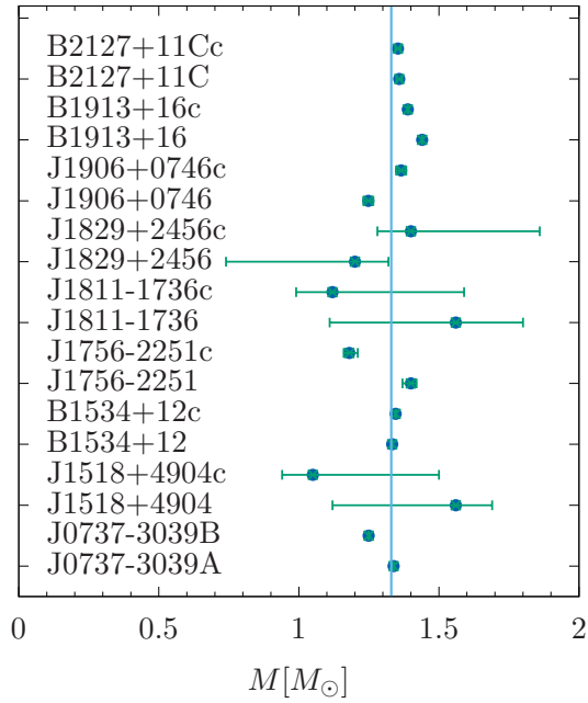
Double Neutron star binaries
