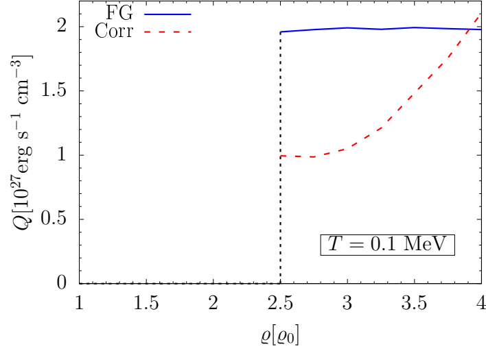
Figure 4.16. Neutrino emissivity at T = 0.1 MeV calculated with expression (4.100), using the correlated \Lambda_{\alpha\beta} and the Fermi gas case. Note that the dUrca threshold takes place at \varrho = 2.5\varrho_0 .
