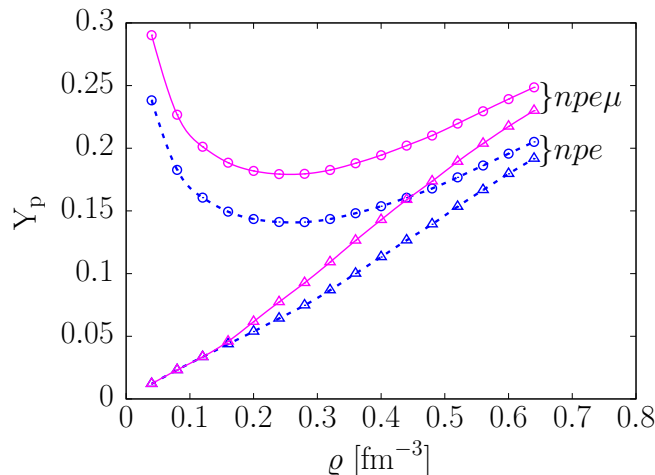
Figure 2.4. Density dependence of the proton fraction in charge-neutral \beta -stable matter. Solid lines marked with triangles and circles correspond to npe\mu matter at T = 0 and 50 MeV, respectively. The same quantities in npe matter are represented by dashed lines.
