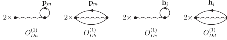
Figure 4.6. First order diagrams contributing to the denominator in Eq. (4.20).
