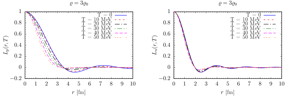
Figure 4.10. Proton (left panel) and neutron (right panel) Slater functions at \varrho = 3\varrho_0 in npe beta-equilibrated matter.
