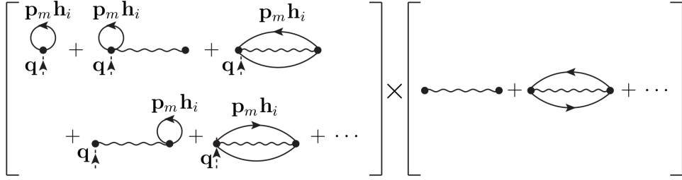
Figure 4.3. Diagrammatic representation of the cluster expansion of the numerator of R_a (4.18).
