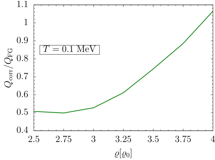
Figure 4.17. Ratio between the curves presented in Fig. 4.16, showing that the quenching of the emissivity varies significantly with density. Also, the maximum quenching takes place at \varrho \sim 2.75\varrho_0 , right after the activation threshold.
