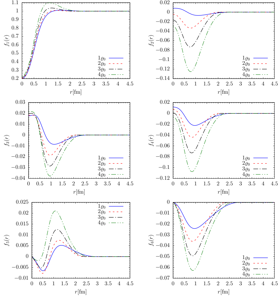
Figure 2.2. Correlation functions that enter the definition of the effective potential (2.52) at \varrho = 1 - 4 \varrho_0 .
