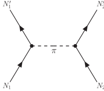
Figure 1.2. Feynman diagram describing the one-pion-exchange process in NN scattering.
