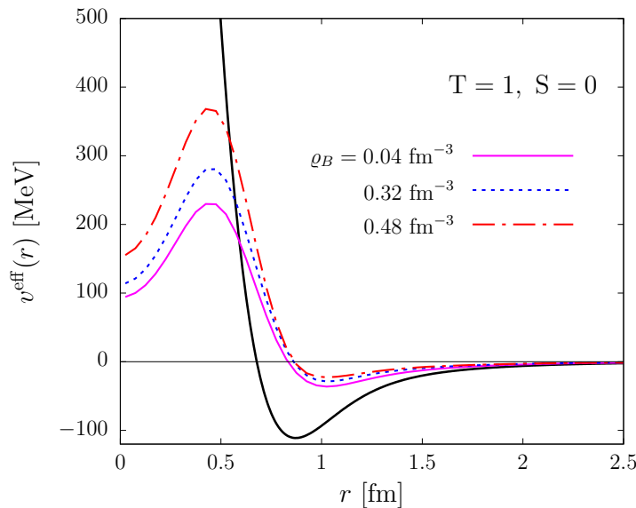
Figure 2.1. Radial dependence of the CBF effective potential in the S = 0 , T = 1 channel. The solid, dashed, and dot-dash lines correspond to baryon number density \varrho = 0.04 , 0.32 and 0.48 \text{ fm}^{-3} . For comparison, the thick solid line shows the bare AV6P potential.
